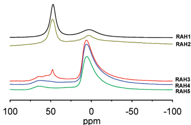
Figure 3. 27 Al NMR spectra of RAH 1, RAH 2, RAH 3, RAH 4, and RAH 5.
