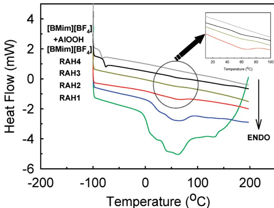
Figure 6. DSC curves of [BMim][BF 4 ]+AIOOH conventional mixture, [BMim][BF 4 ], RAH 1, RAH 2, RAH 3, and RAH 4. (Inset) Expanded view of [BMim][BF 4 ]+AIOOH conventional mixture, [BMim][BF 4 ], RAH 3, and RAH 4, marked with a circle.
